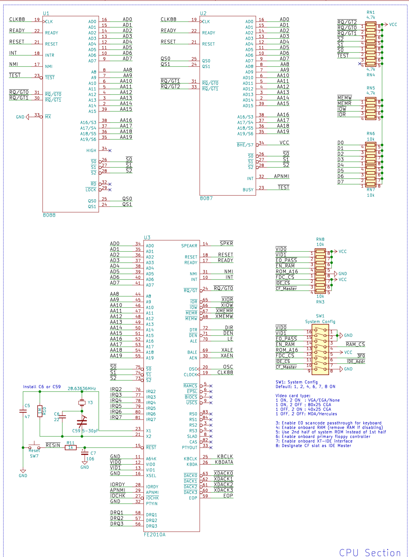
CPU Section
