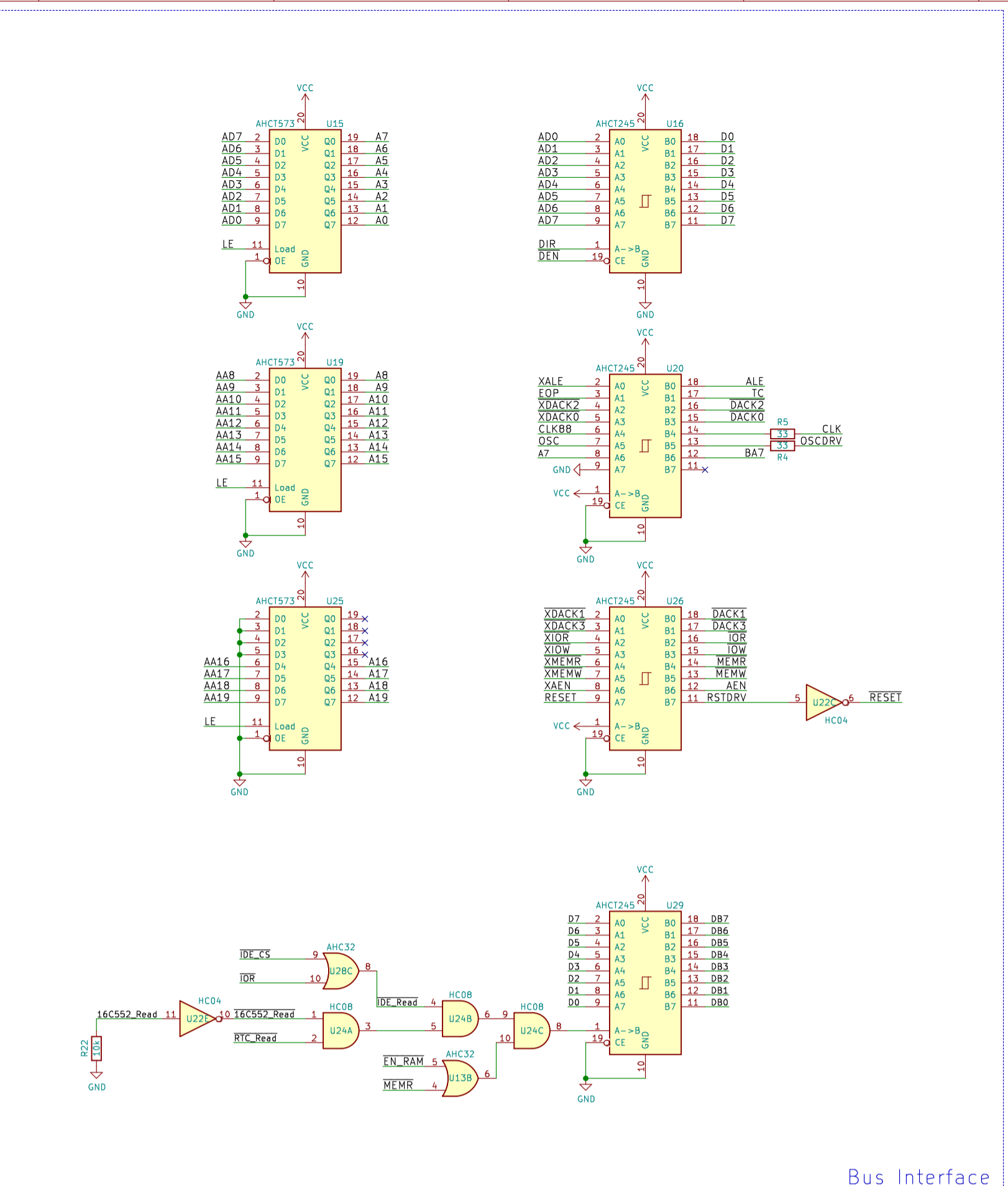
Bus Interface
