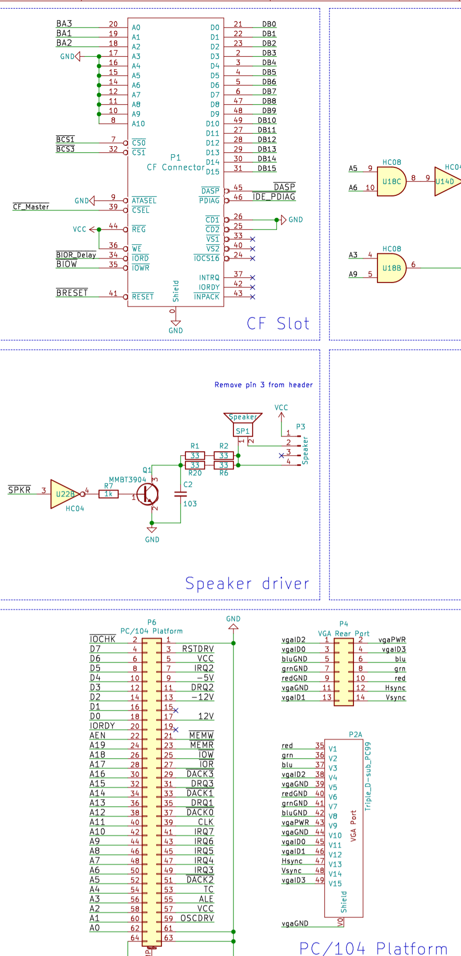
PC/104 Platform
