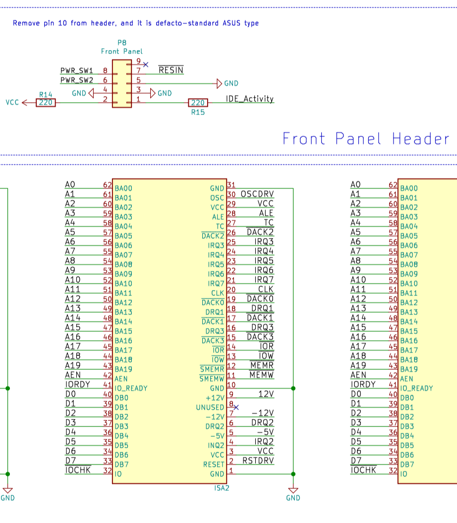
PC/104 Platform
